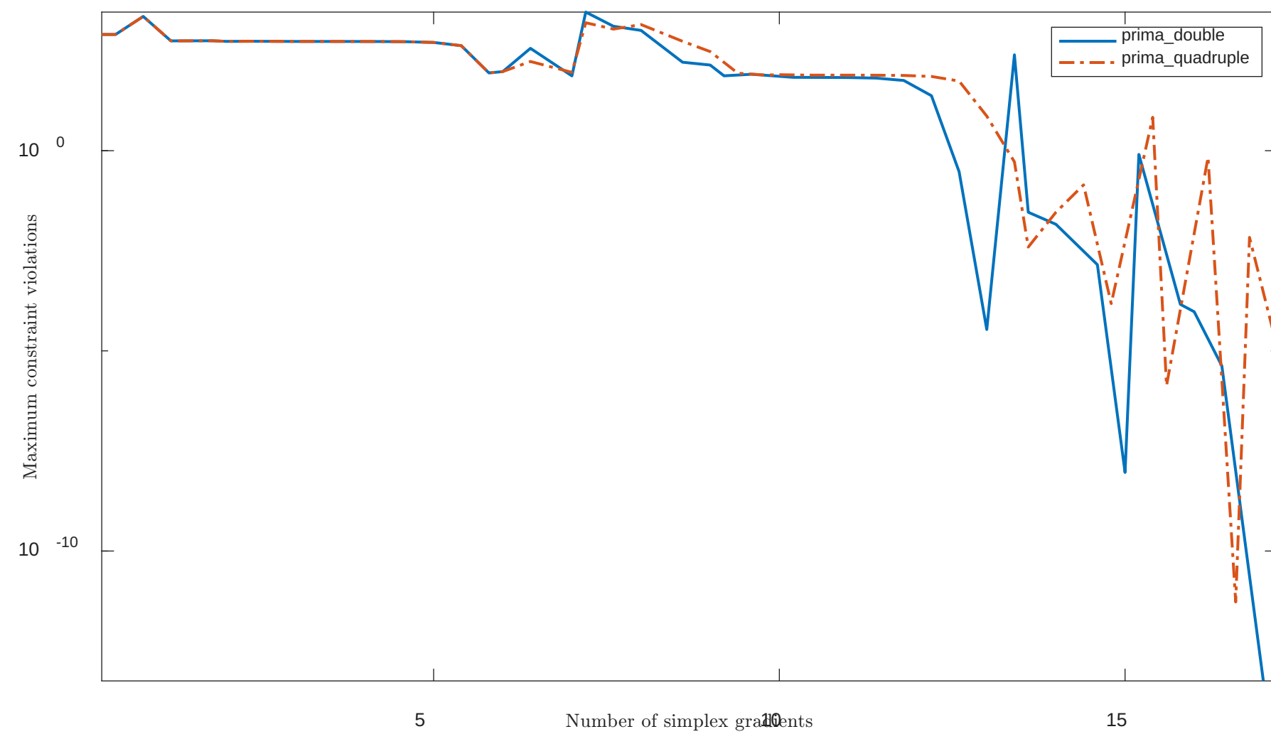
Solving "HS75" with "plain" feature
