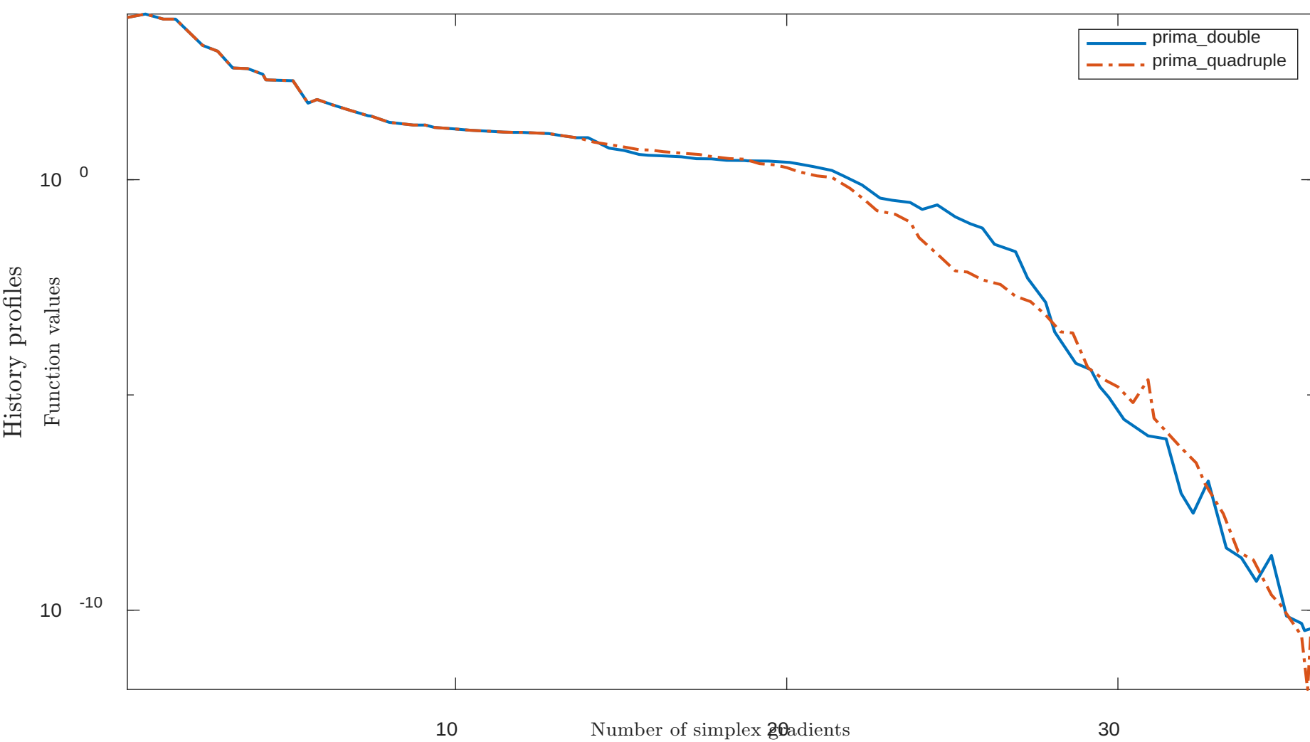
Solving "LIARWHD" with "plain" feature
