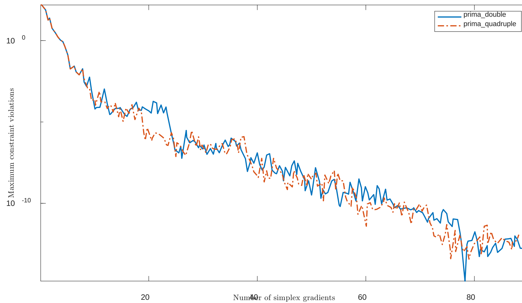
Solving "LUKVLE3" with "plain" feature
