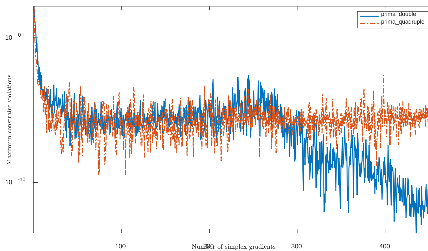
Solving "LUKVL4" with "plain" feature
