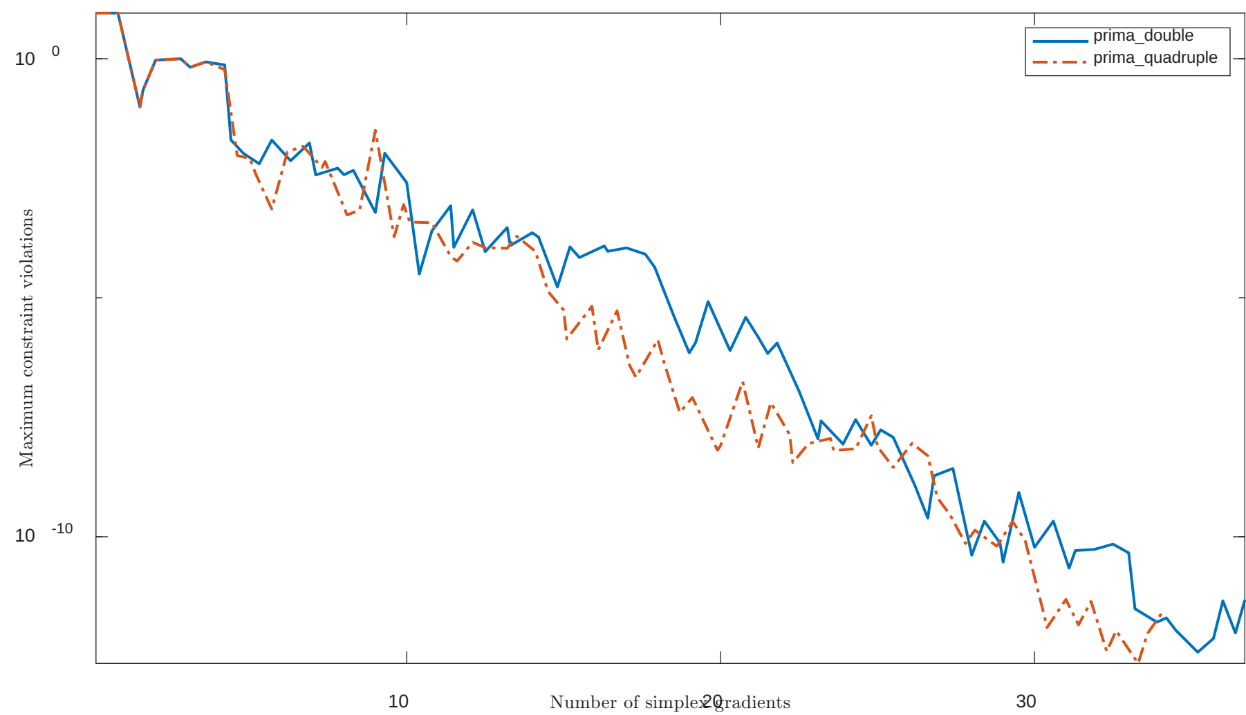
Solving "LUKVLE6" with "plain" feature
