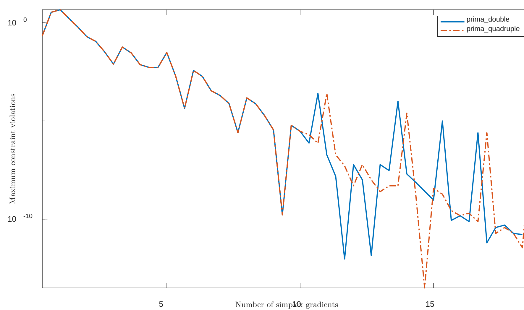
Solving "MARATOS" with "plain" feature
