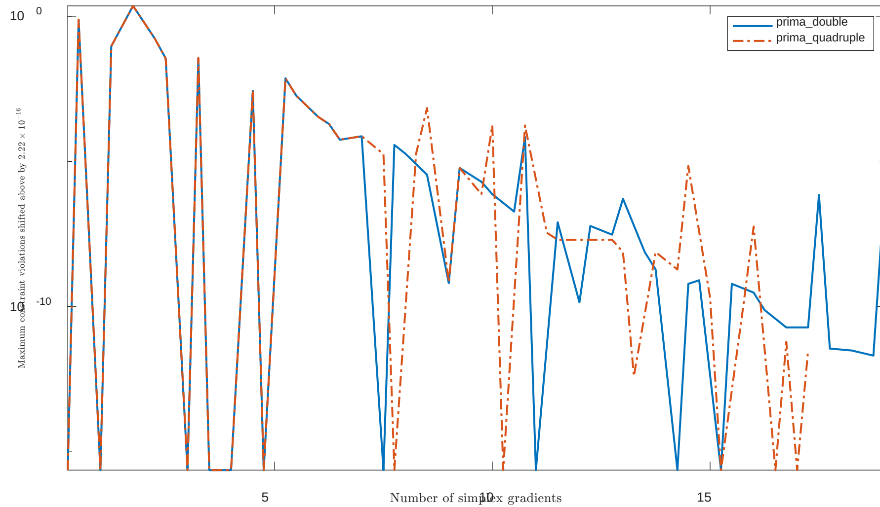
Solving "MIFFLIN1" with "plain" feature
