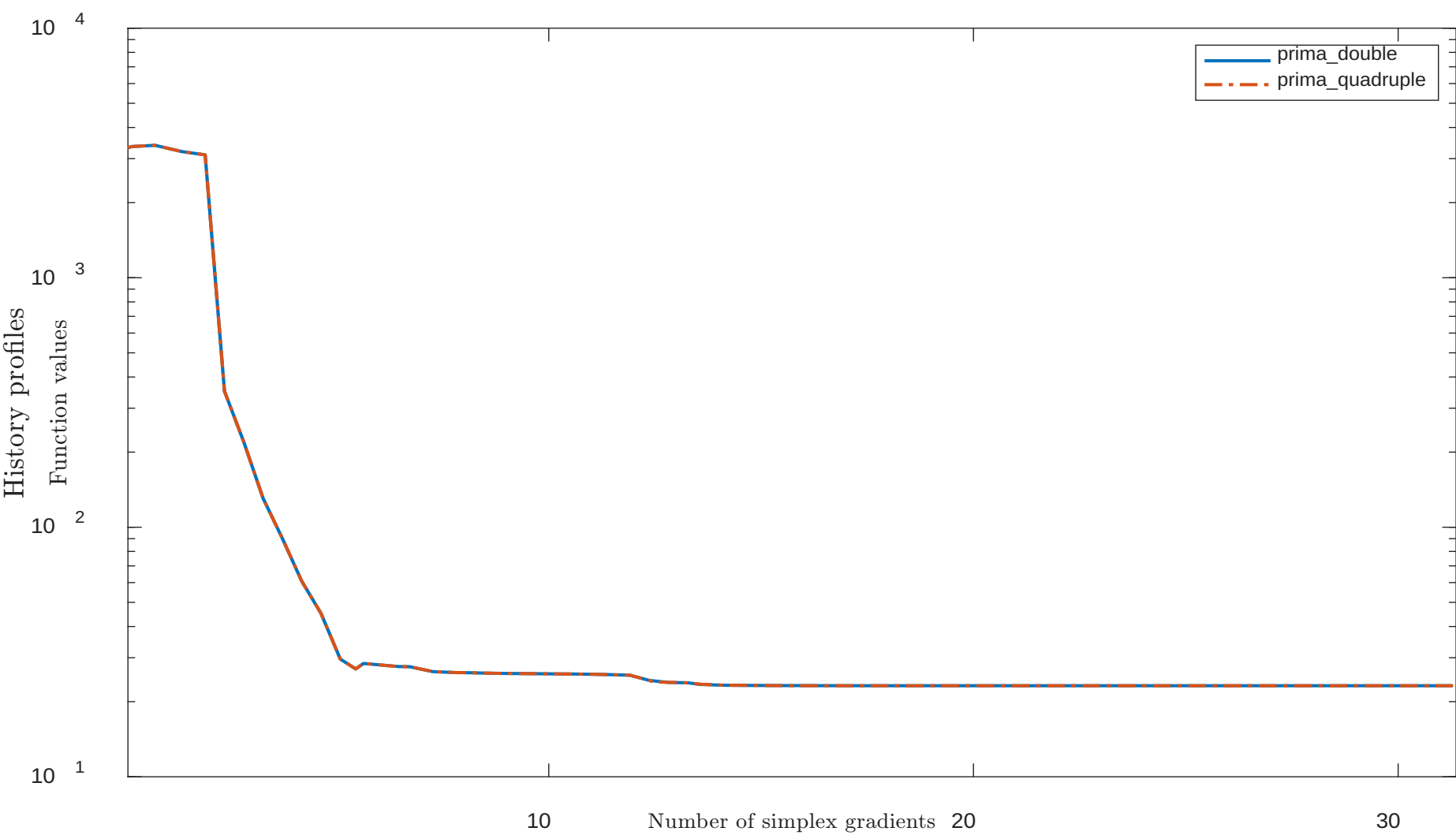
Solving “NONCVXUN” with “plain” feature
