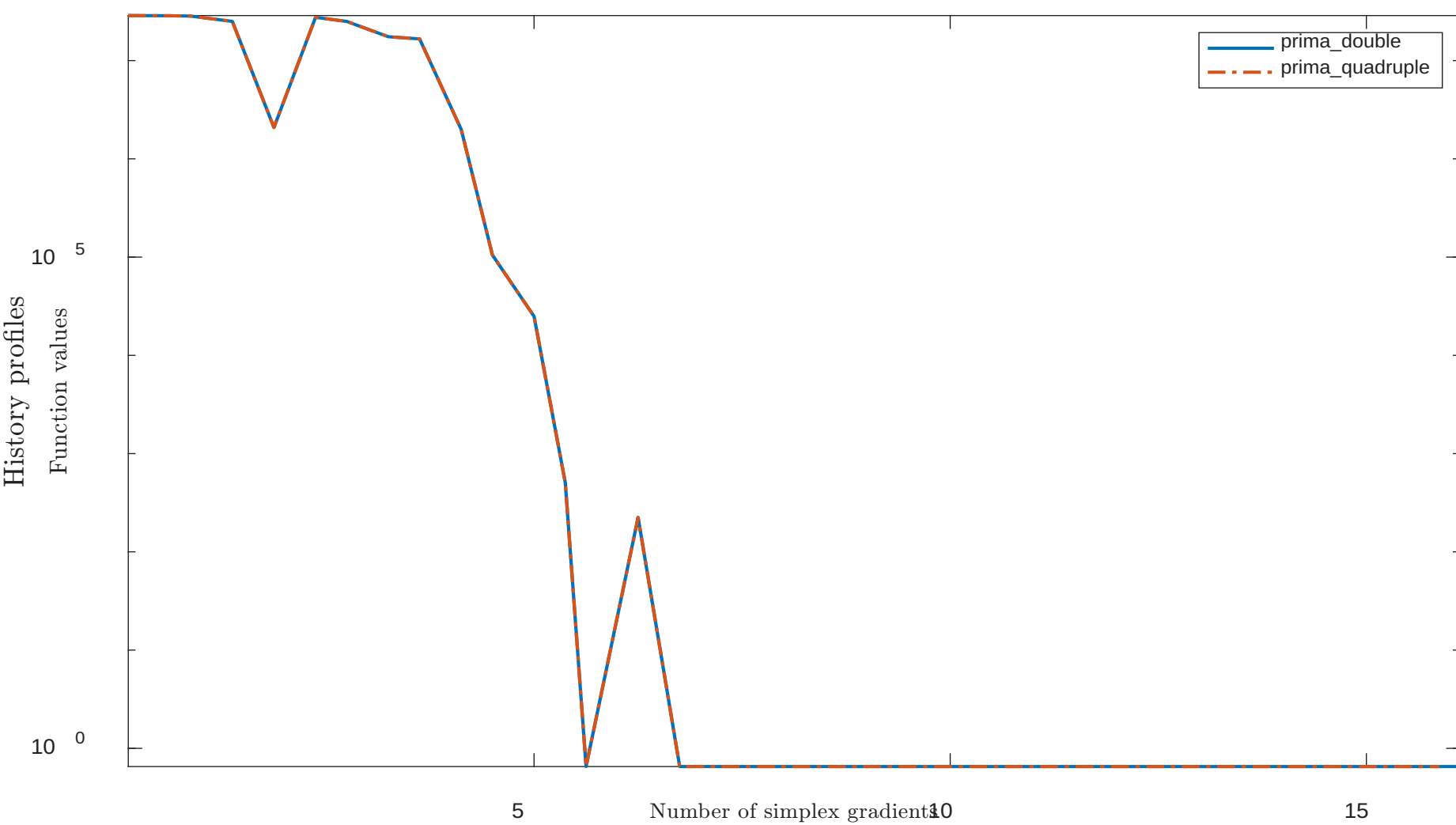
Solving “PALMER1D” with “plain” feature
