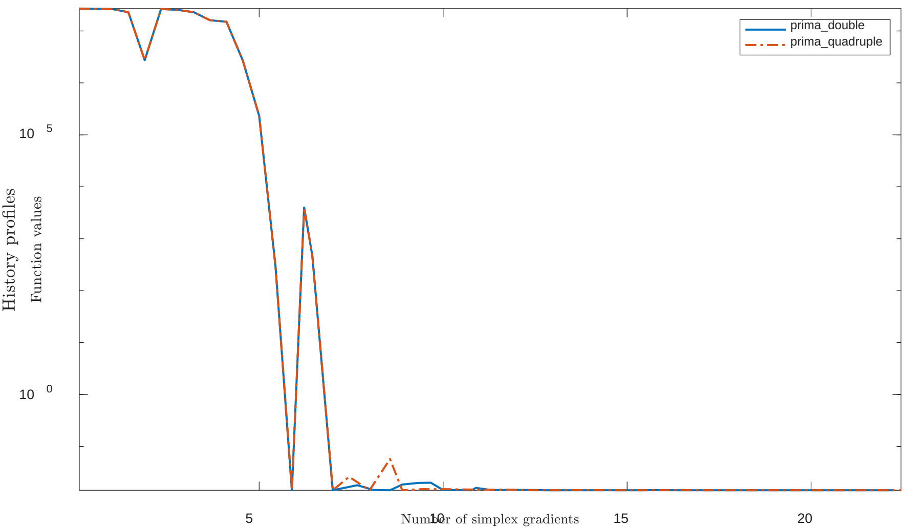
Solving "PALMER2C" with "plain" feature
