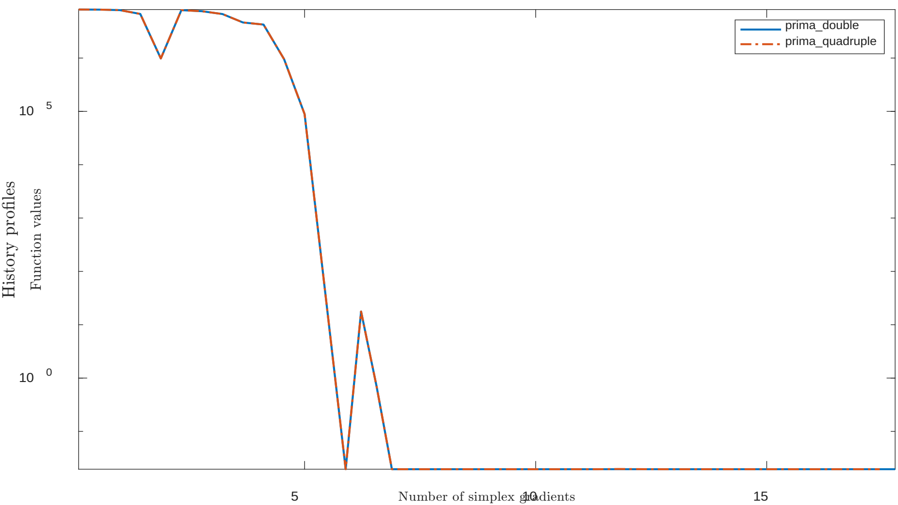
Solving “PALMER3C” with “plain” feature
