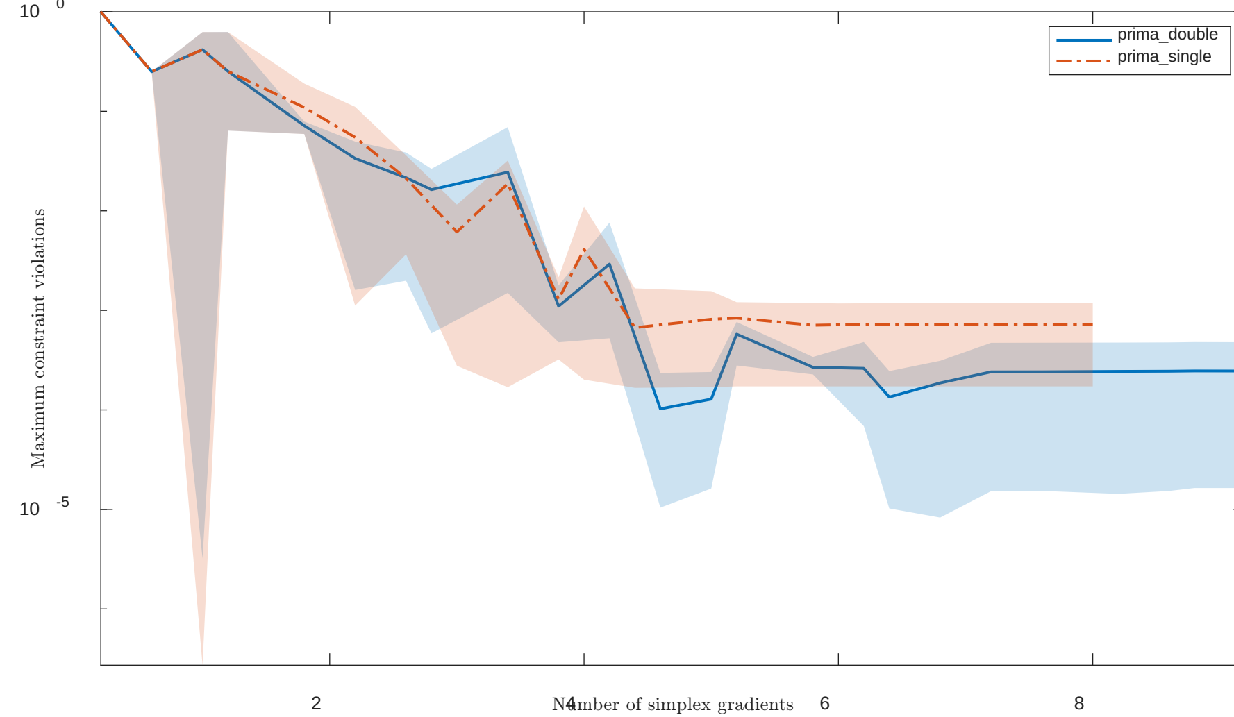
Solving "ALLINITA" with "noisy" feature
