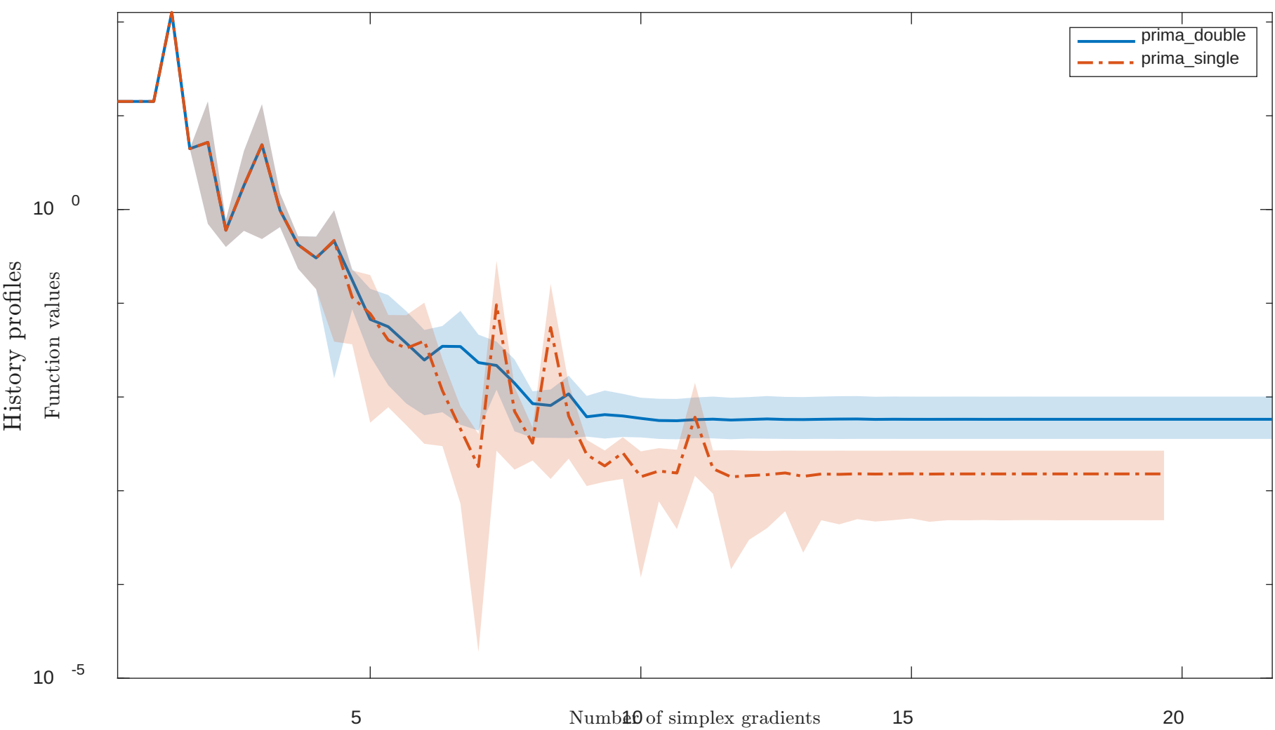
Solving “BEALE” with “noisy” feature
