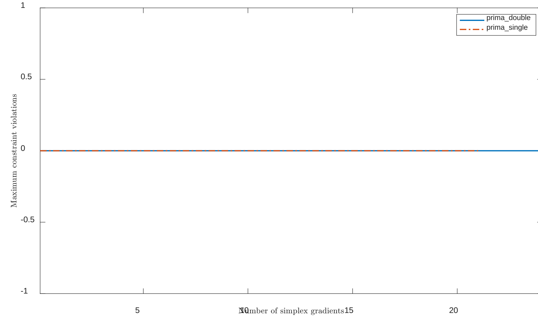
Solving "BRATU1D" with "noisy" feature
