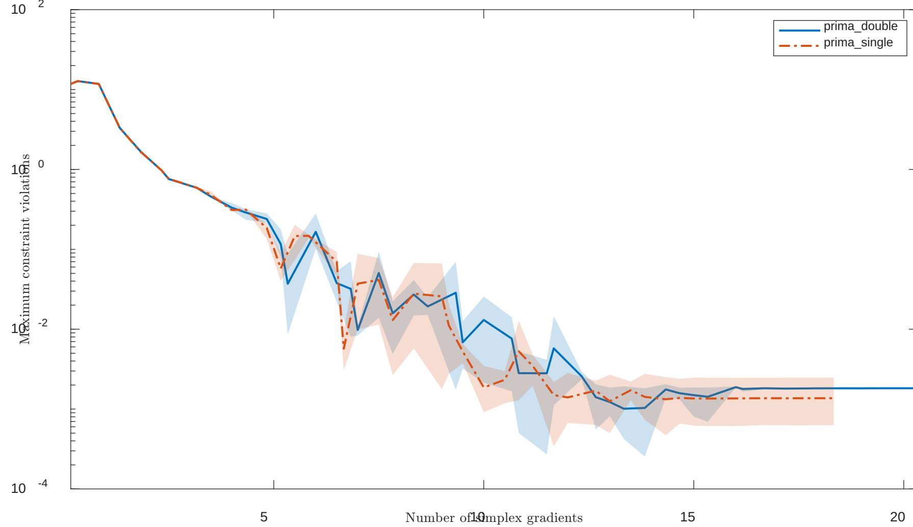
Solving “BT11” with “noisy” feature
