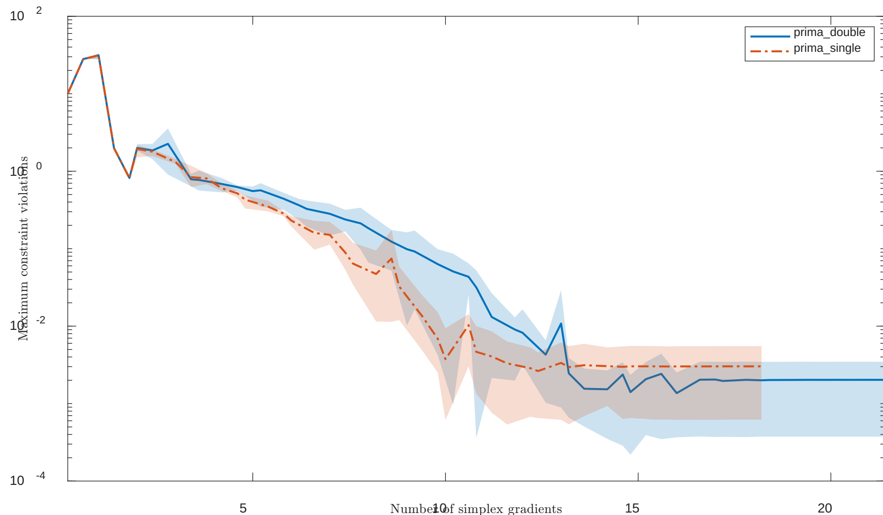
Solving “BT9” with “noisy” feature
