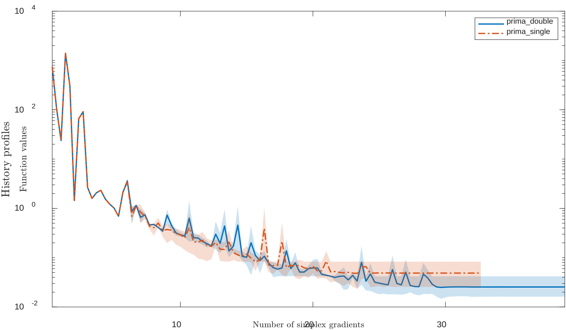
Solving “CUBE” with “noisy” feature
