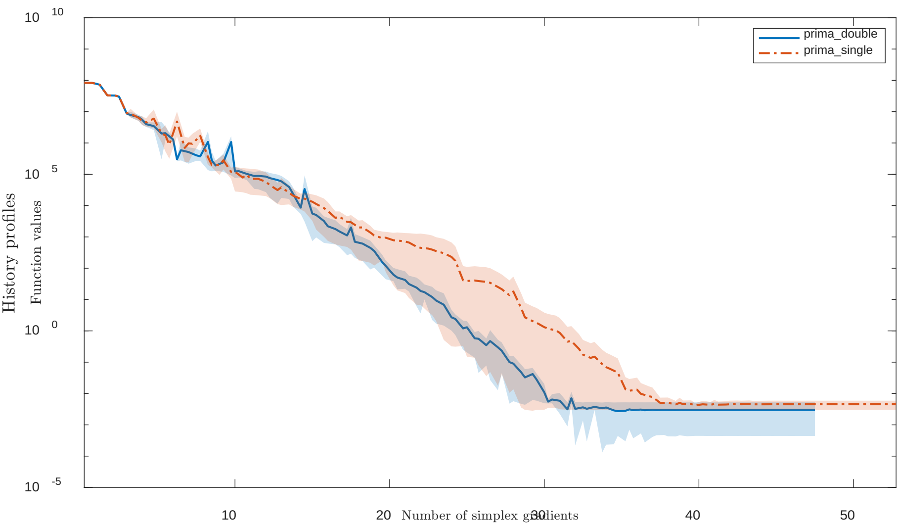
Solving “DENSCHND” with “noisy” feature
