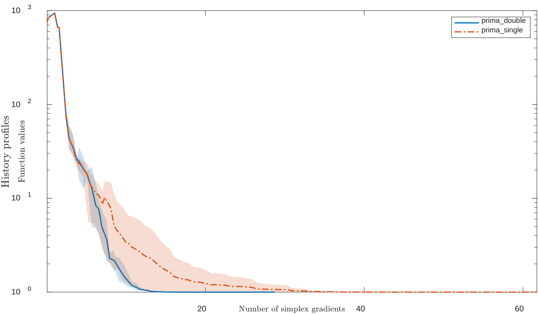
Solving “DIXMAAND” with “noisy” feature
