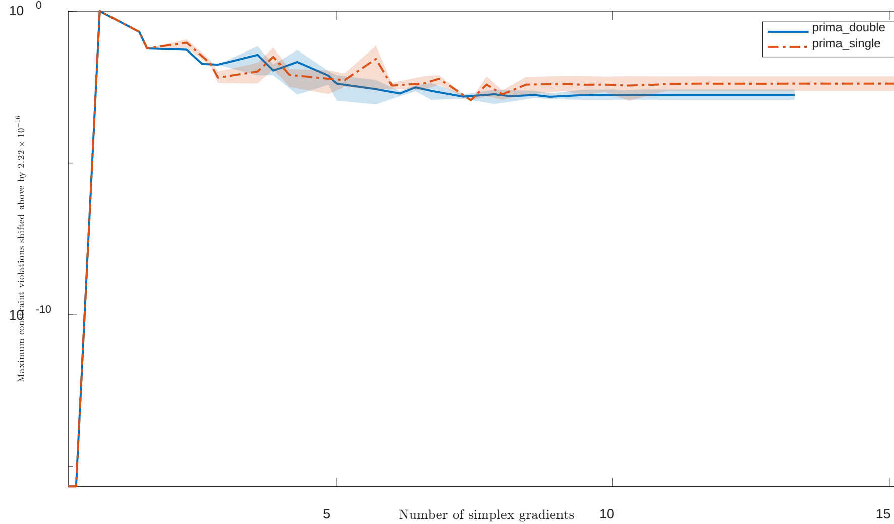
Solving "EIGENB2" with "noisy" feature
