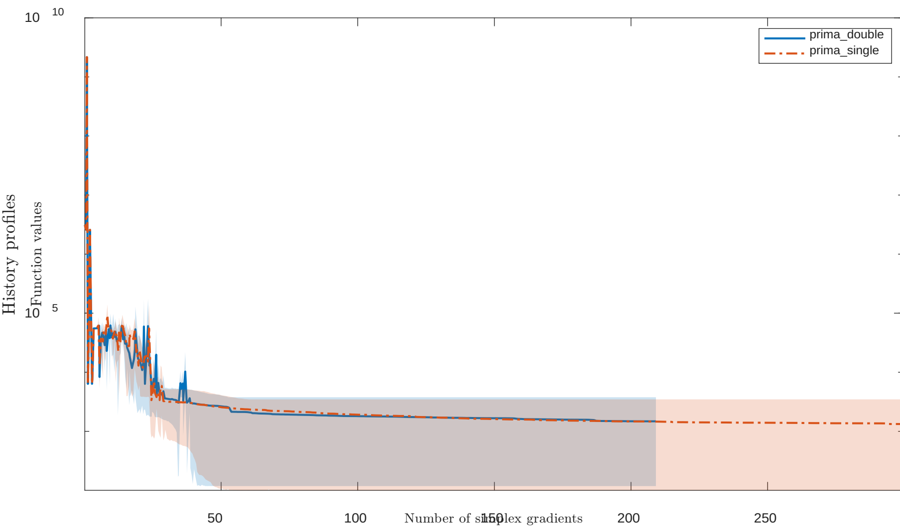
Solving “HAHN1LS” with “noisy” feature
