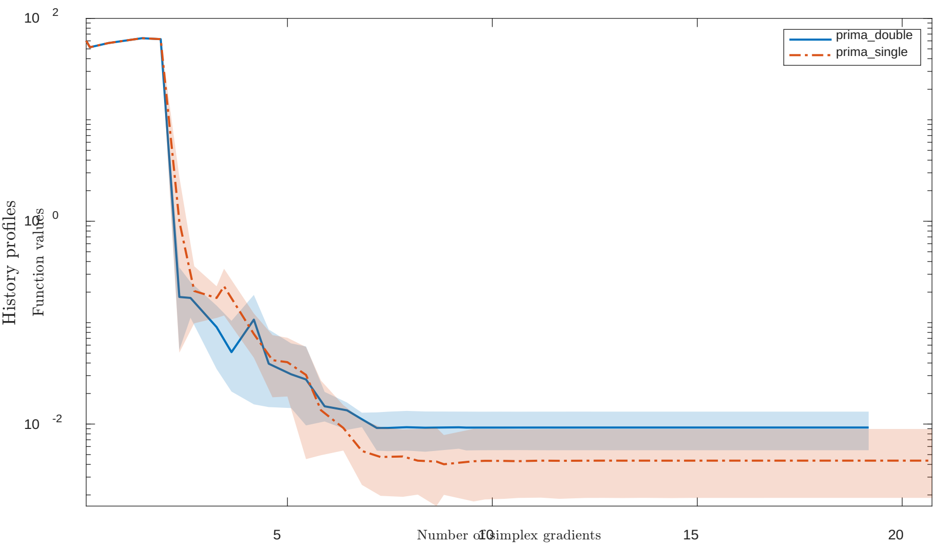
Solving “HILBERTA” with “noisy” feature
