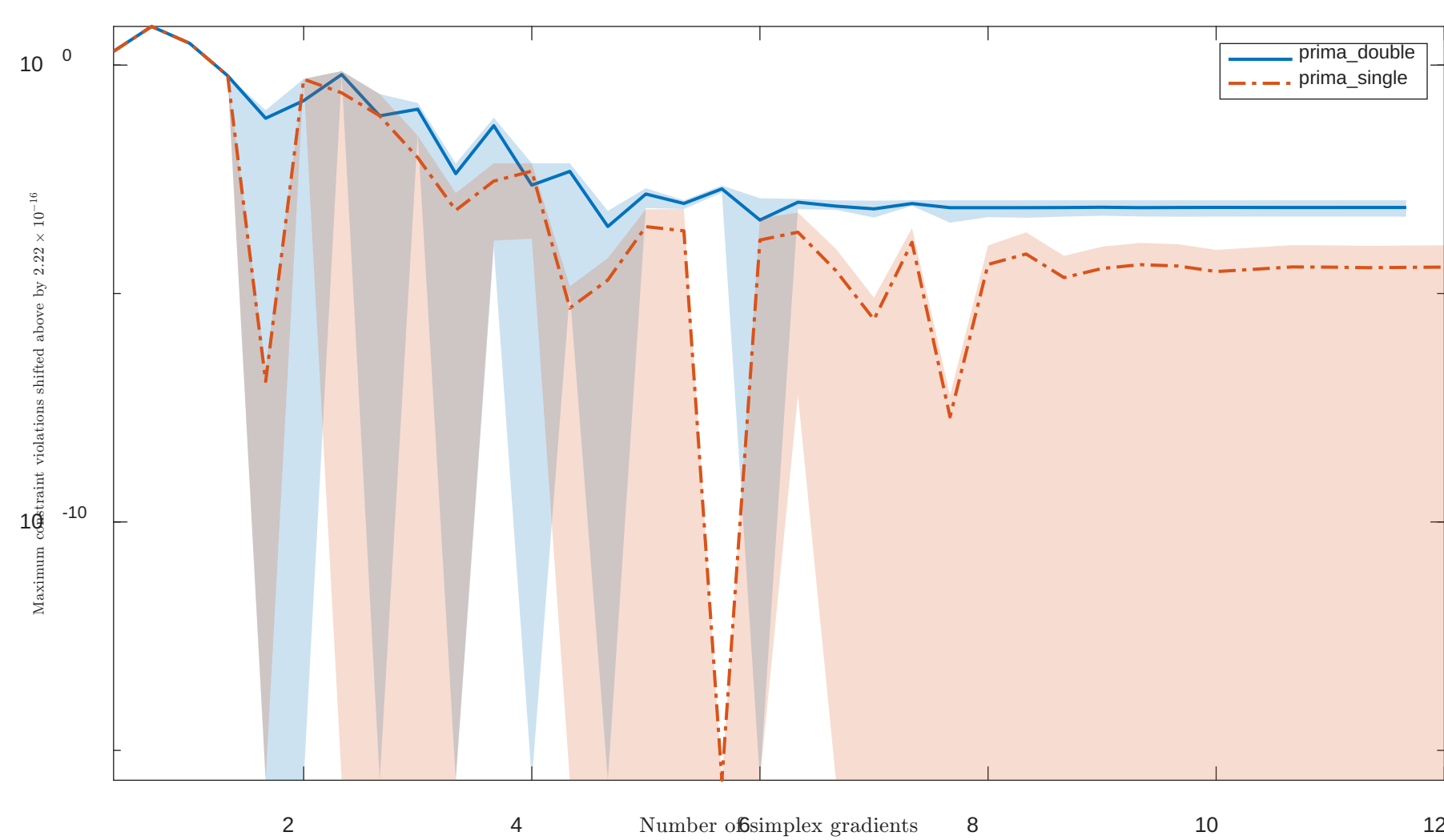
Solving "HS22" with "noisy" feature
