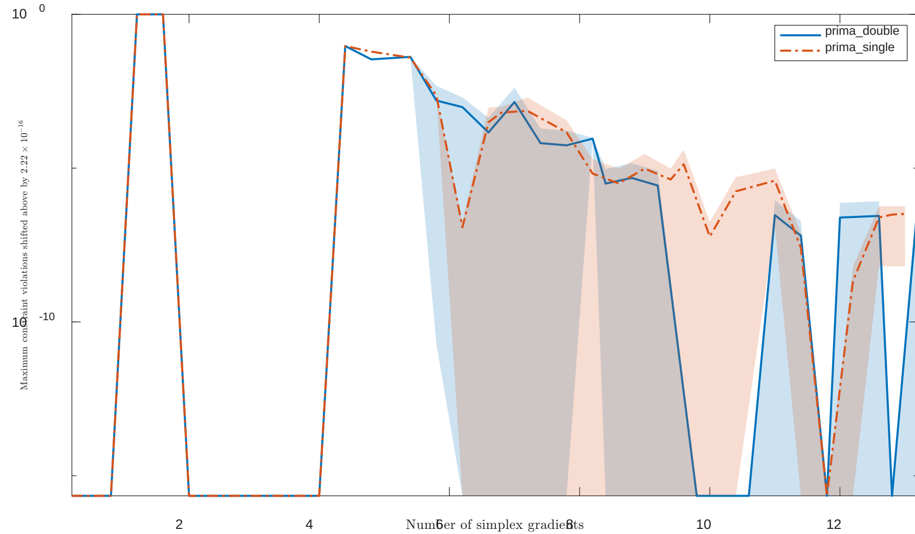
Solving “HS44” with “noisy” feature
