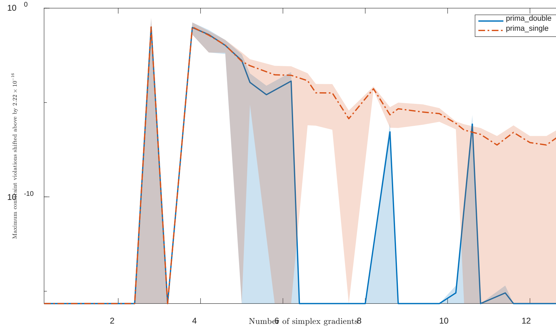
Solving “HS44NEW” with “noisy” feature
