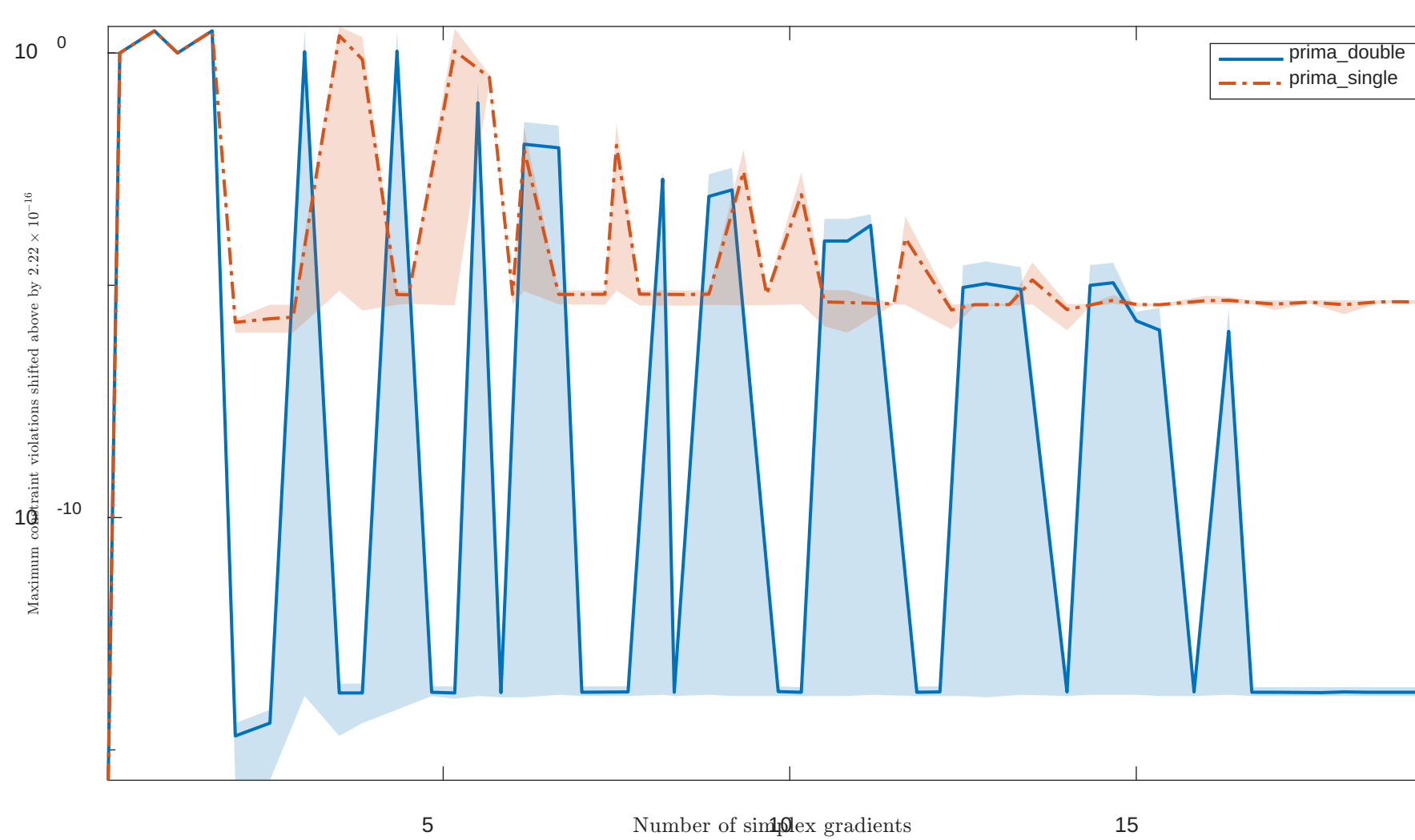
Solving "HS50" with "noisy" feature
