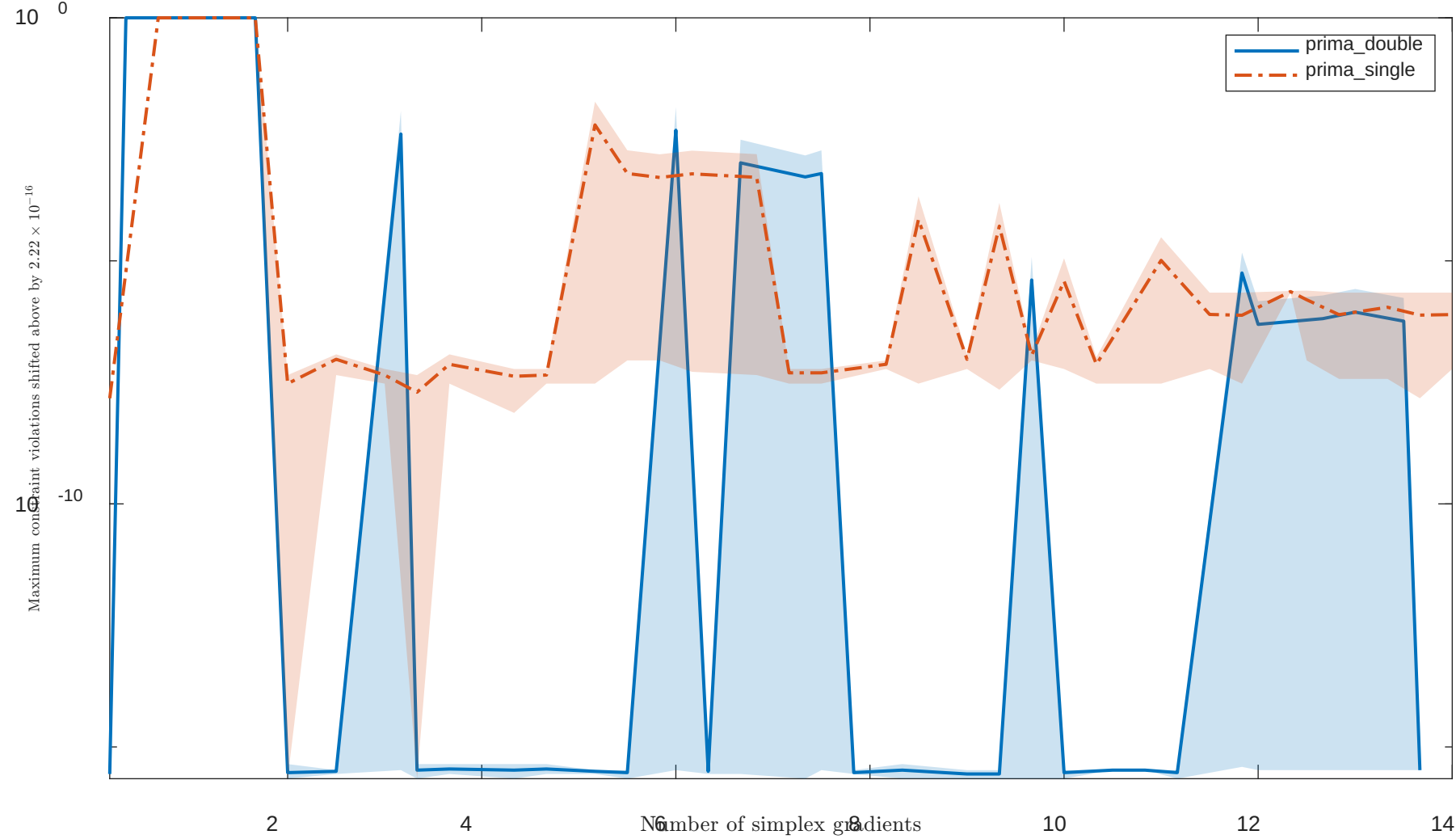
Solving "HS53" with "noisy" feature
