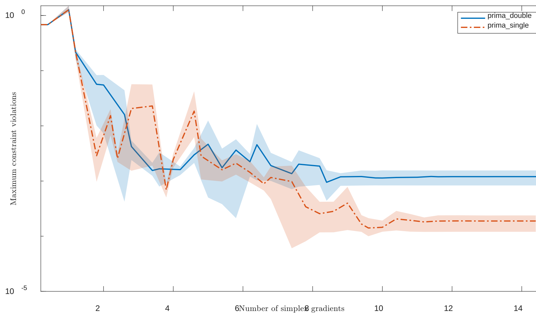
Solving "HS69" with "noisy" feature
