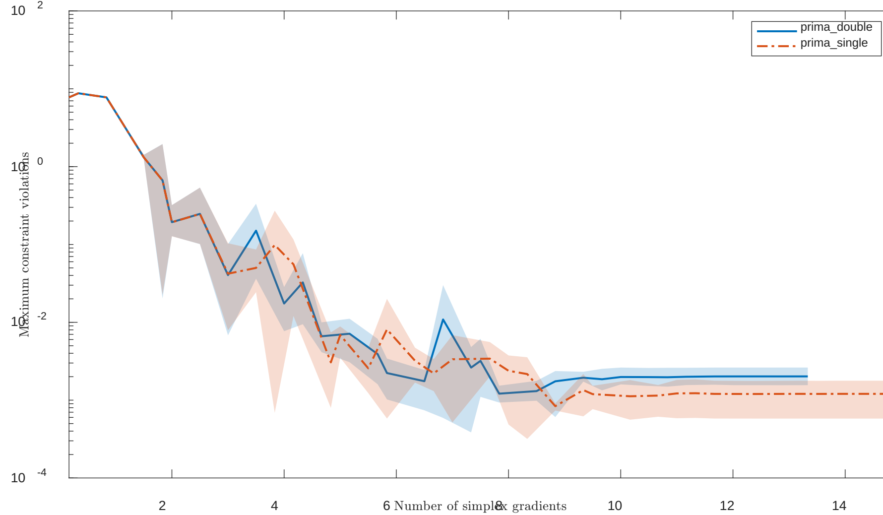
Solving "HS79" with "noisy" feature
