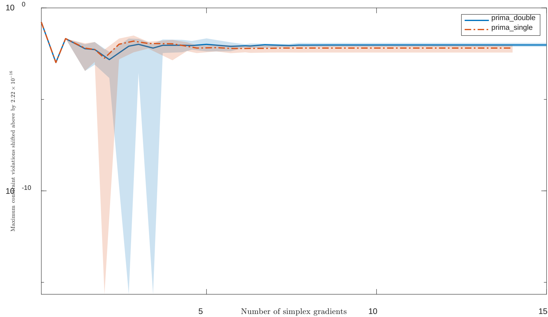
Solving “HS92” with “noisy” feature
