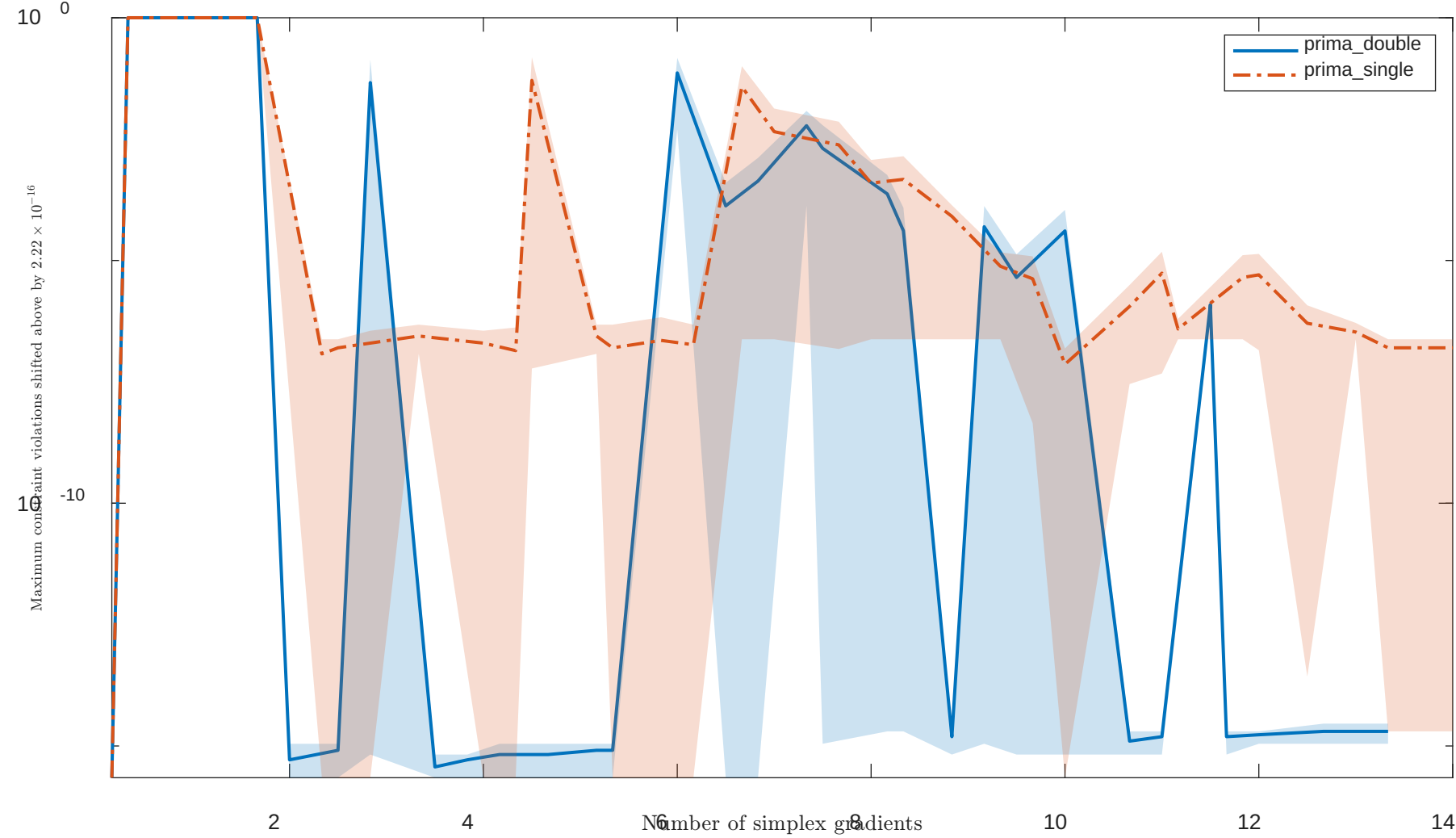
Solving "LSNNODOC" with "noisy" feature
