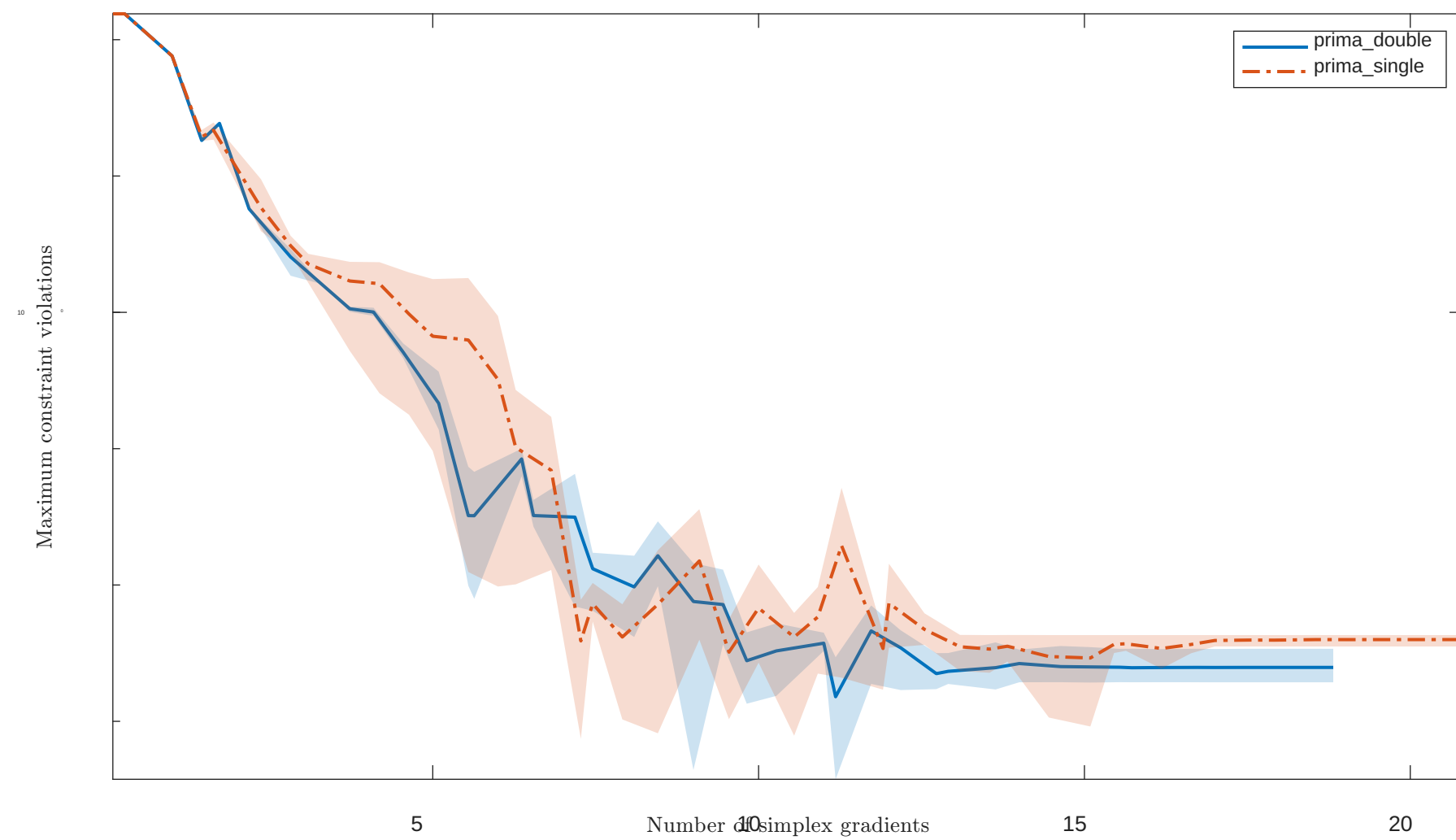
Solving "LUKVLE3" with "noisy" feature
