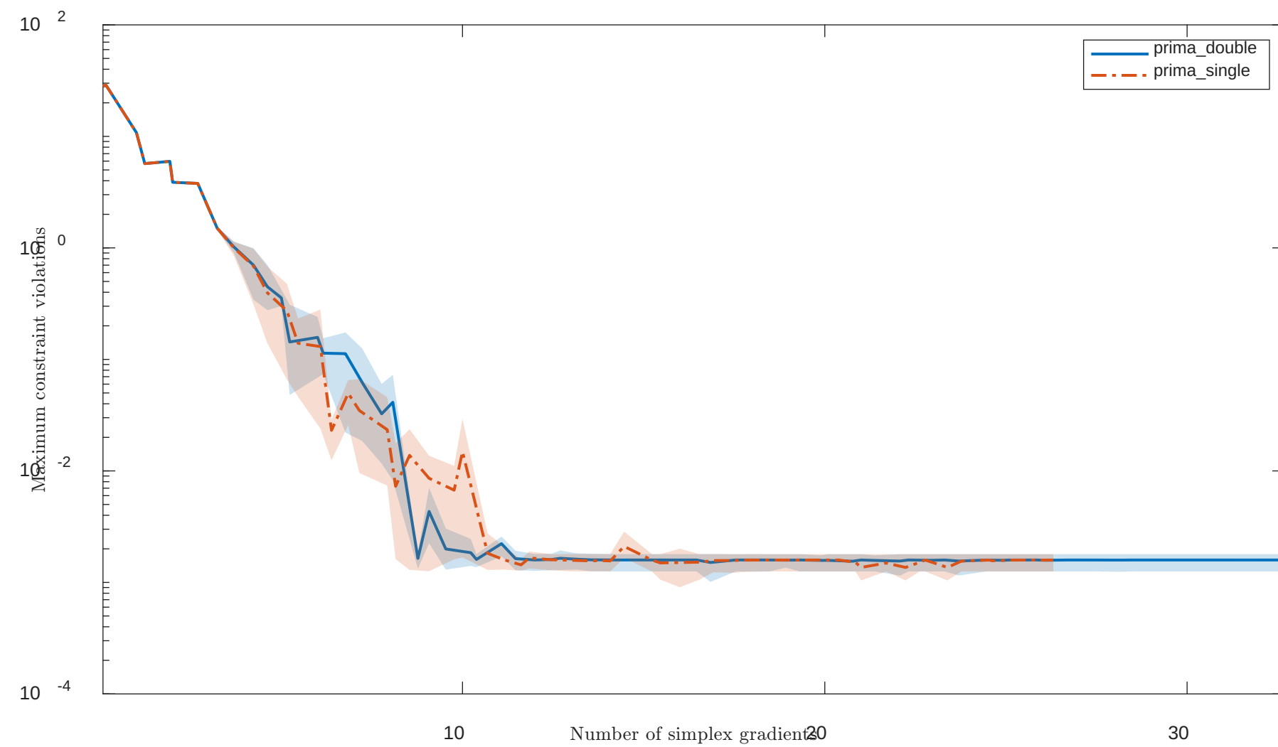
Solving "LUKVLE5" with "noisy" feature
