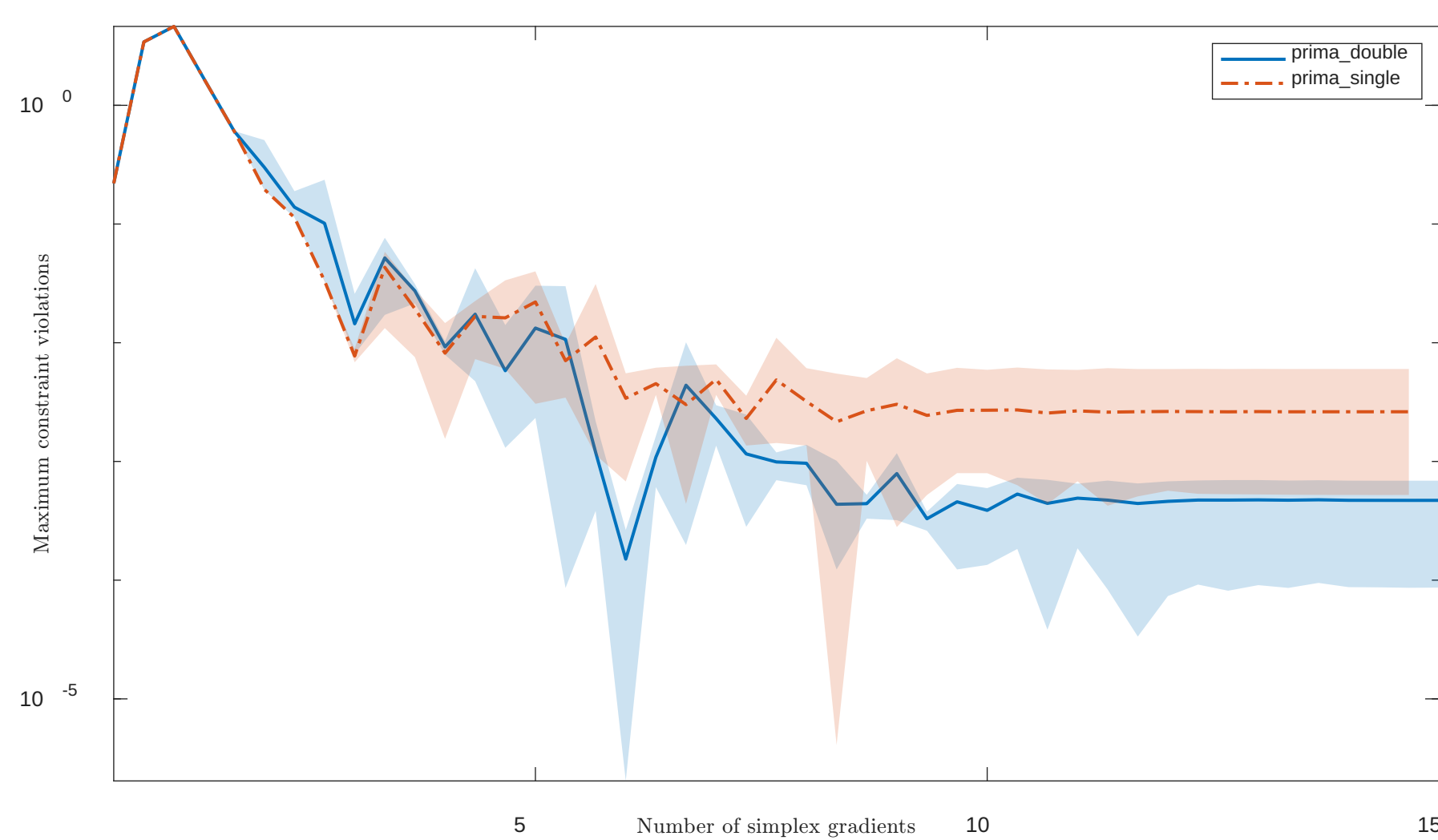
Solving "MARATOS" with "noisy" feature
