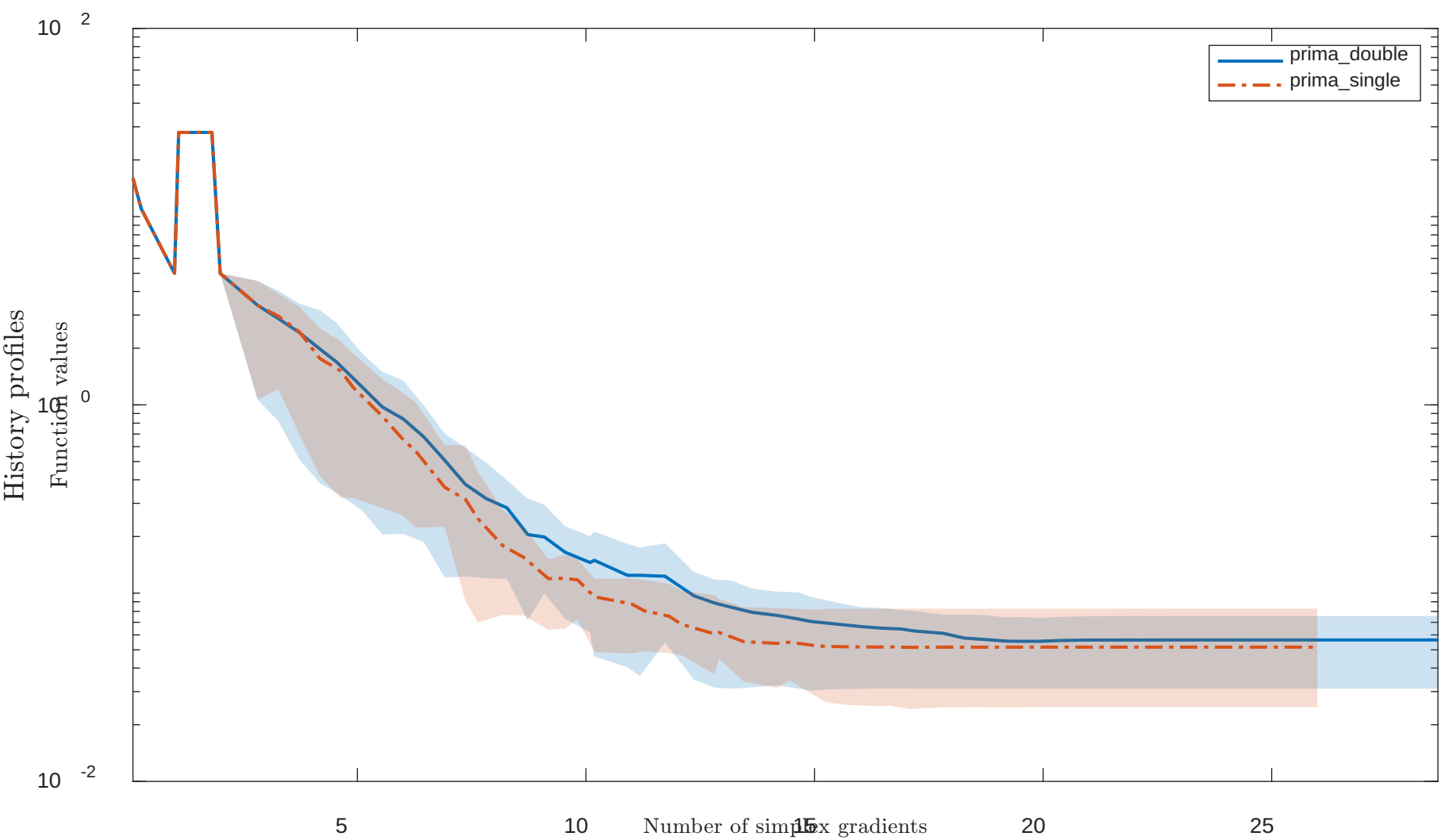
Solving “NONDQUAR” with “noisy” feature
