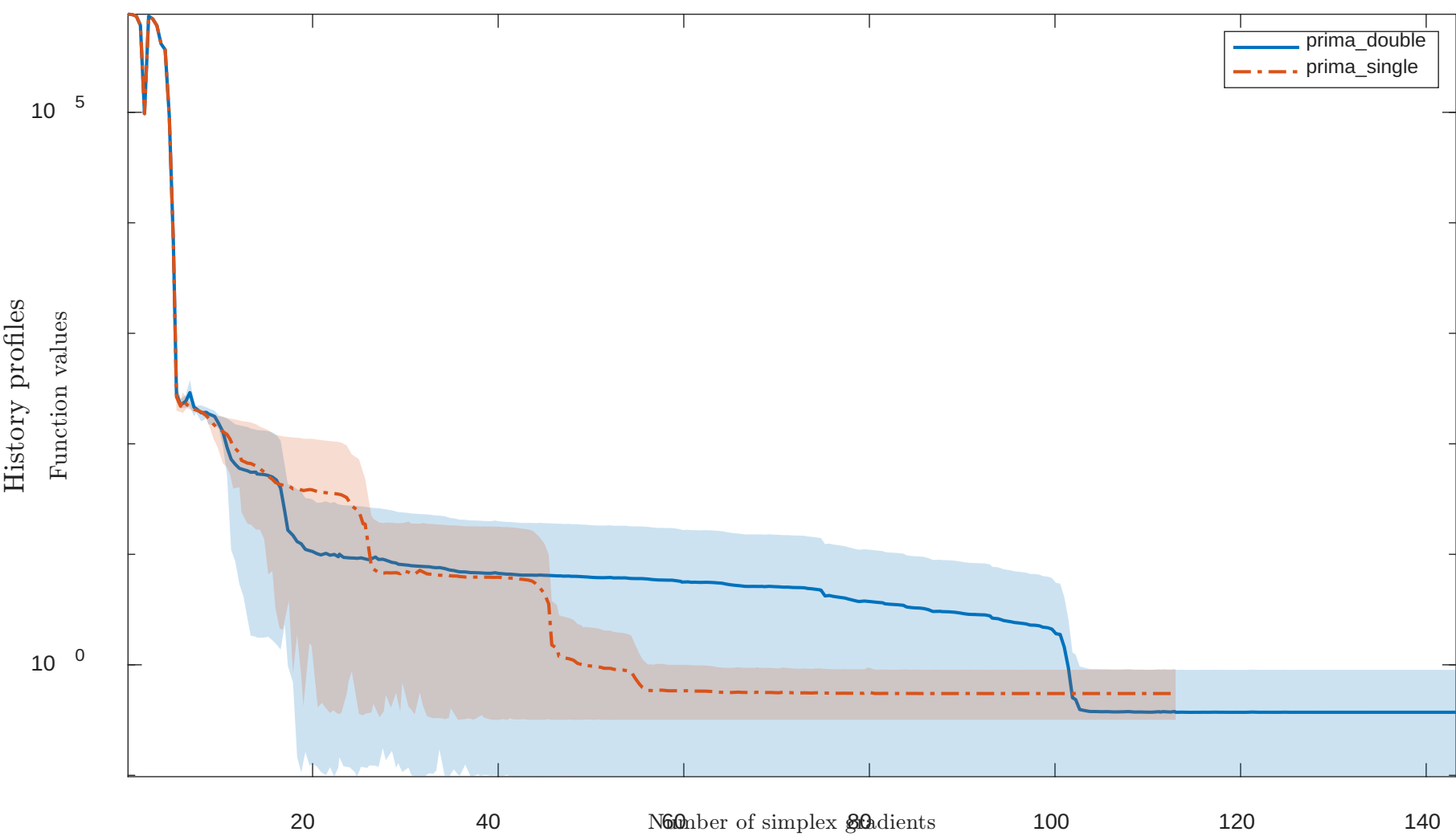
Solving "PALMER6C" with "noisy" feature
