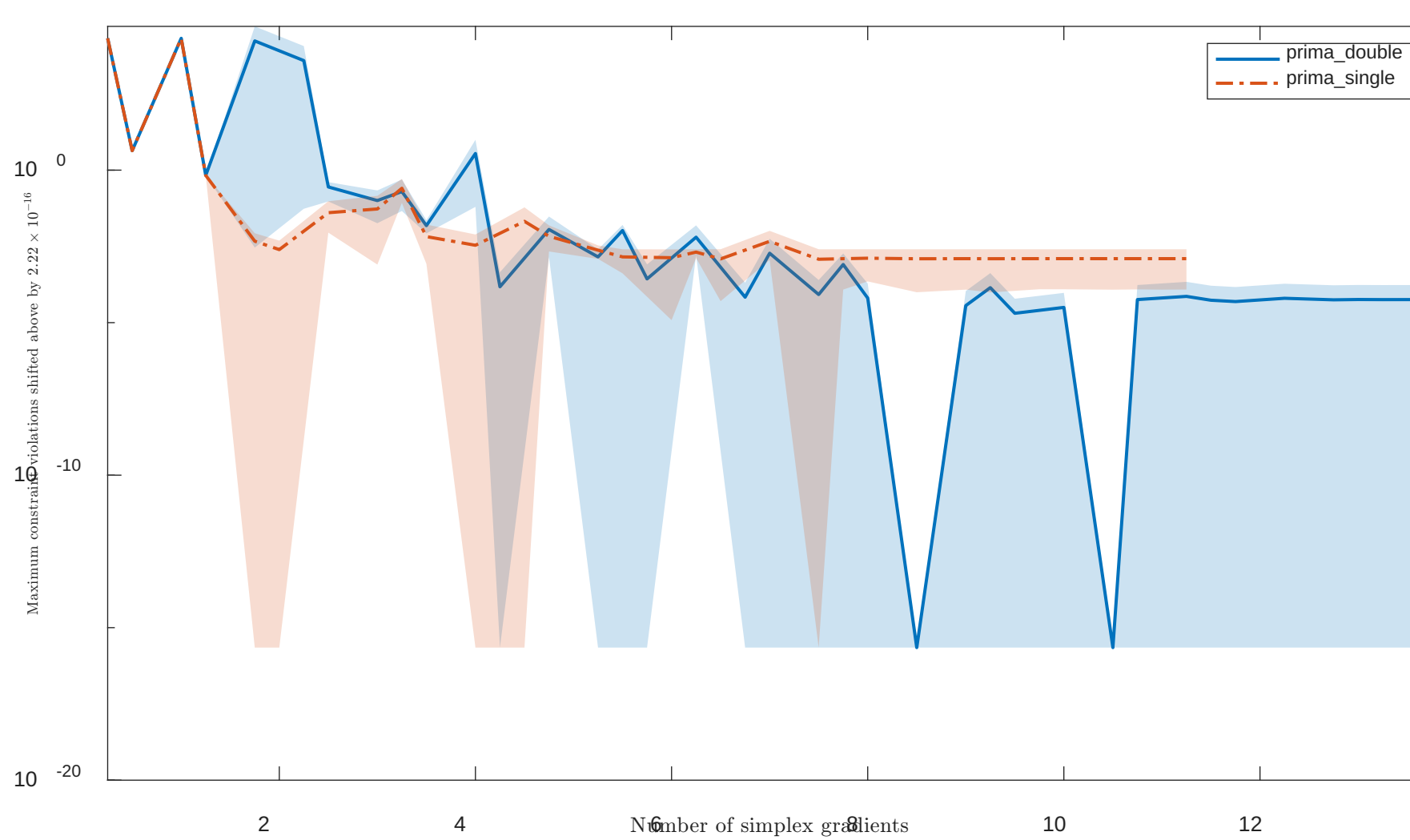
Solving "POLAK4" with "noisy" feature
