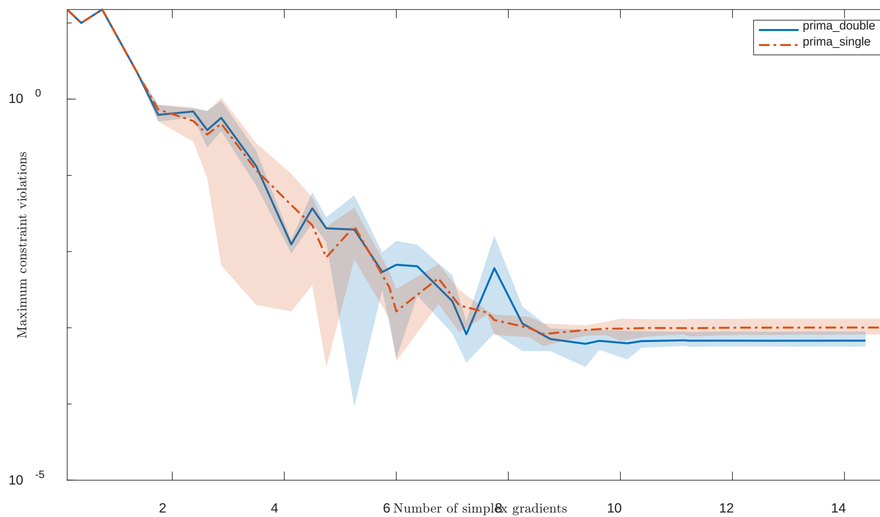
Solving "S365" with "noisy" feature
