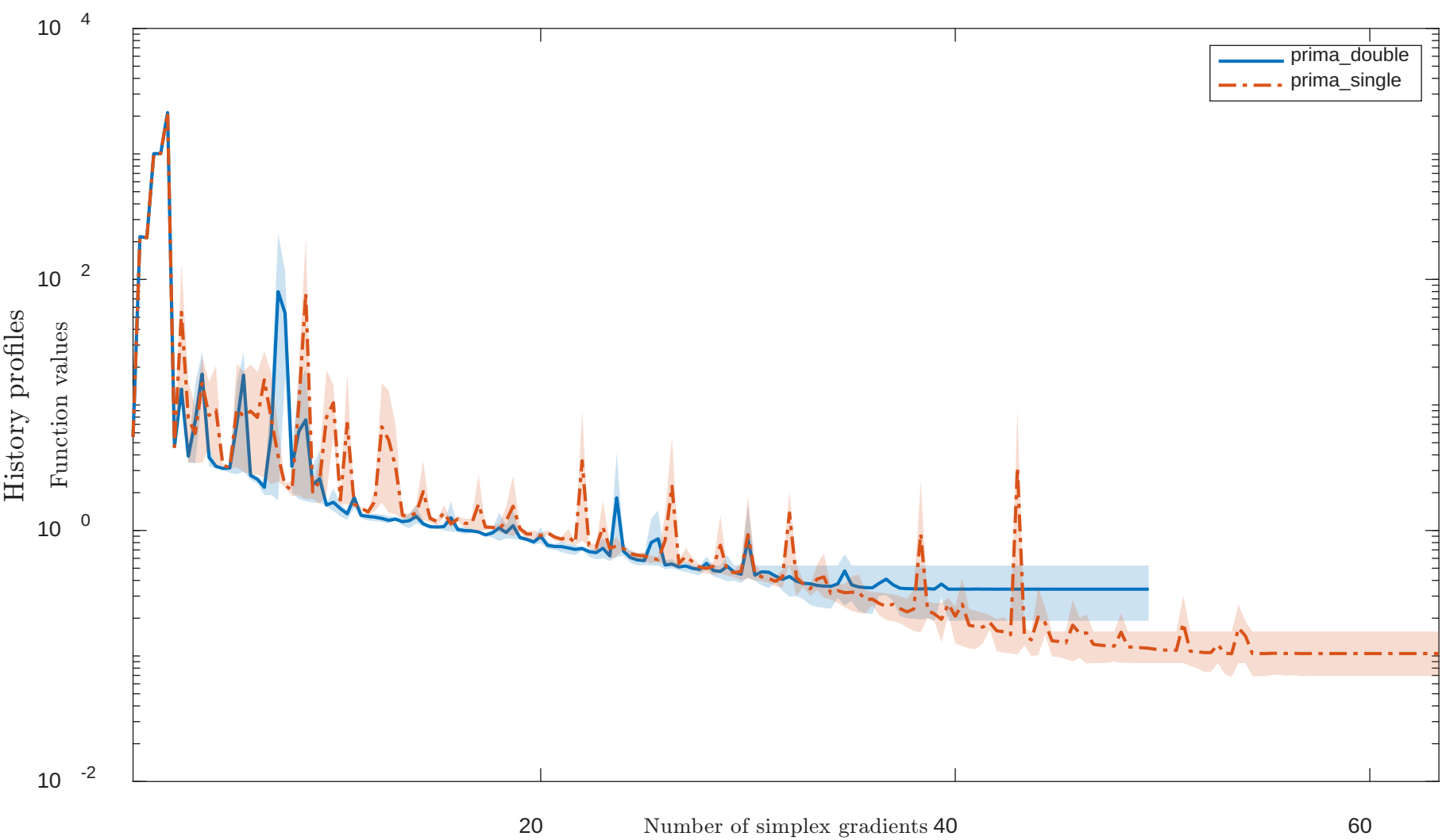
Solving “SINEVAL” with “noisy” feature
