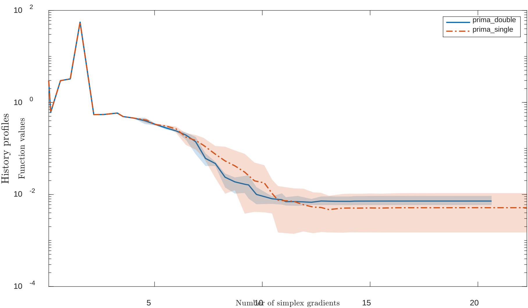
Solving “TRIGON1” with “noisy” feature
