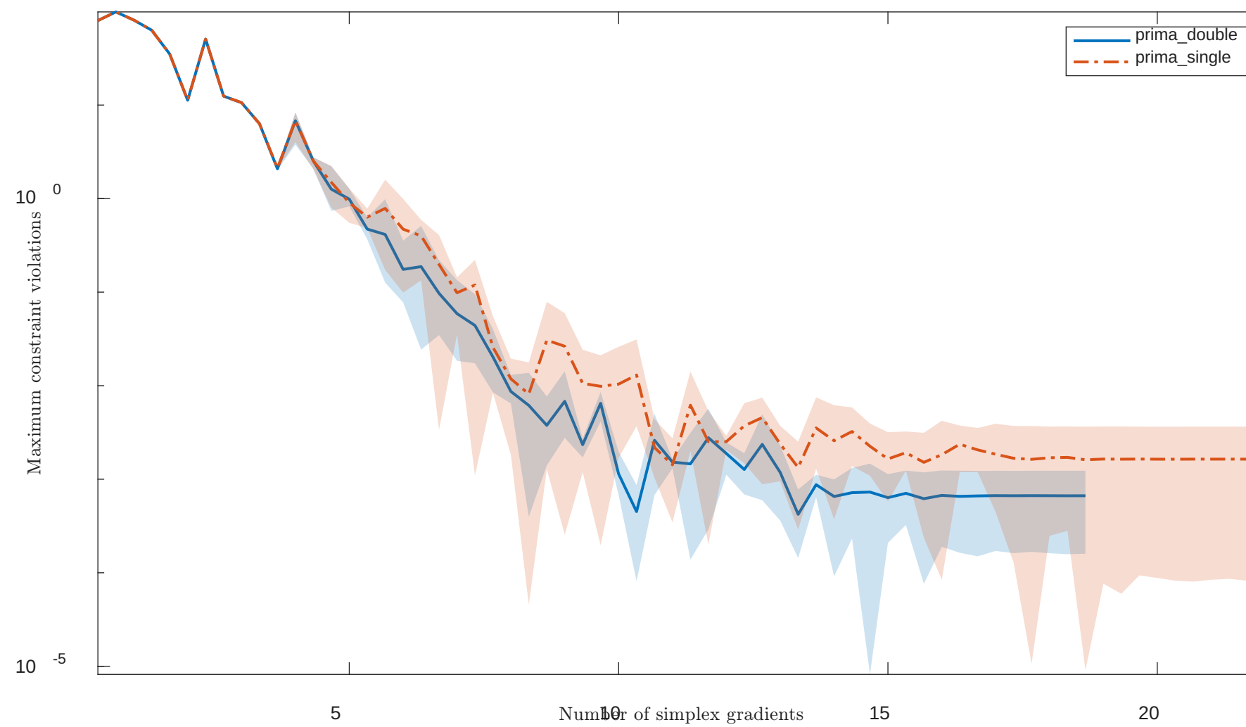
Solving “TRYmB” with “noisy” feature
