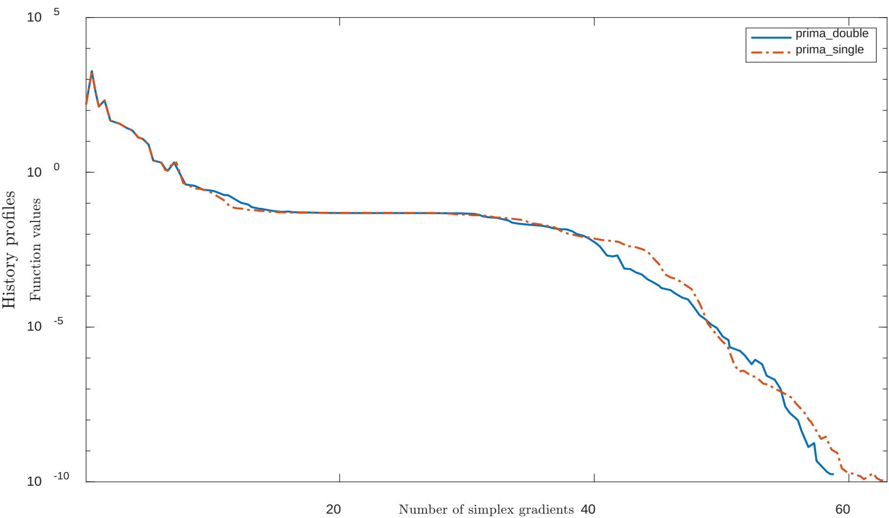
Solving “BRYBND” with “plain” feature
