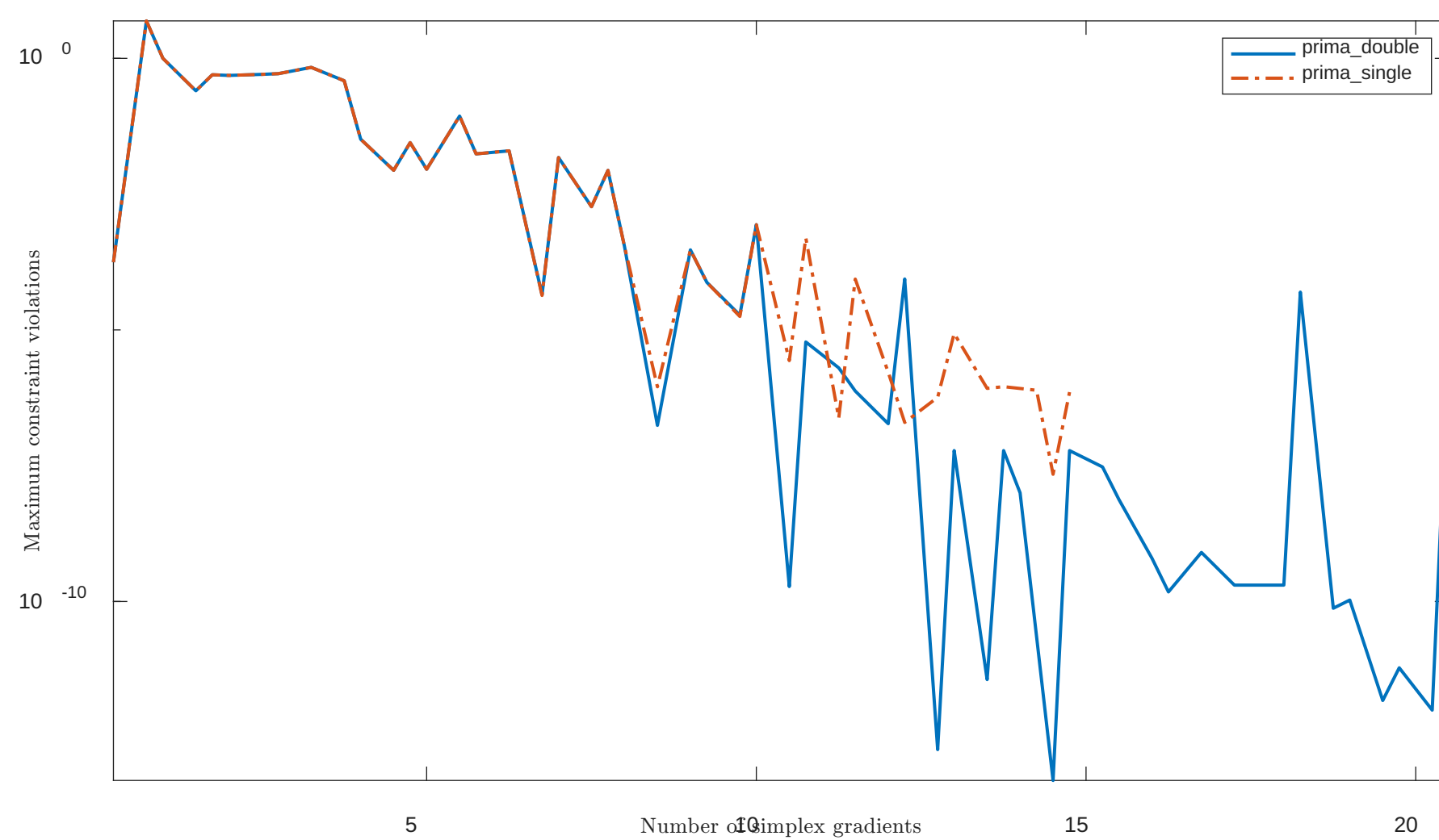
Solving "BT4" with "plain" feature
