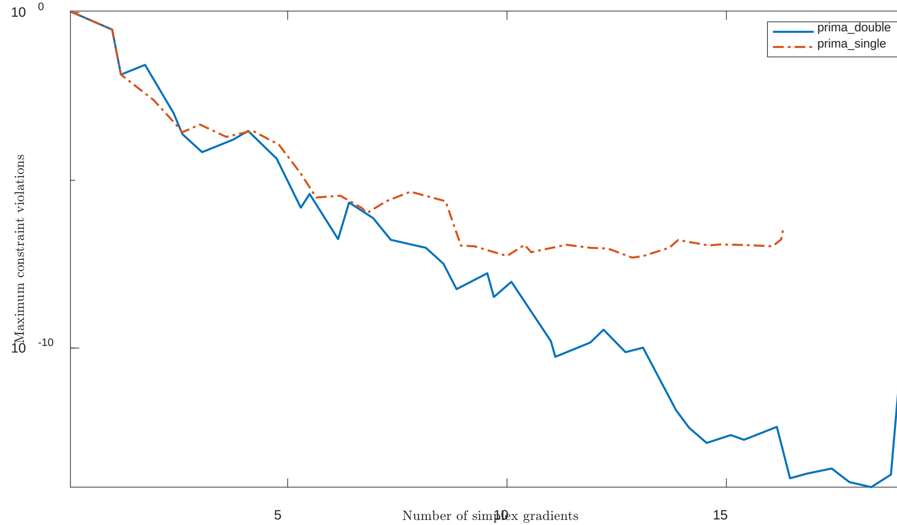
Solving "DTC5" with "plain" feature
