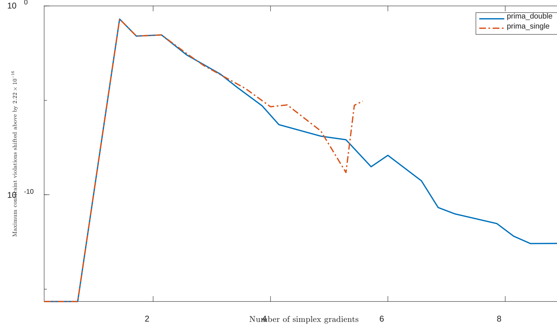
Solving "EIGENACO" with "plain" feature
