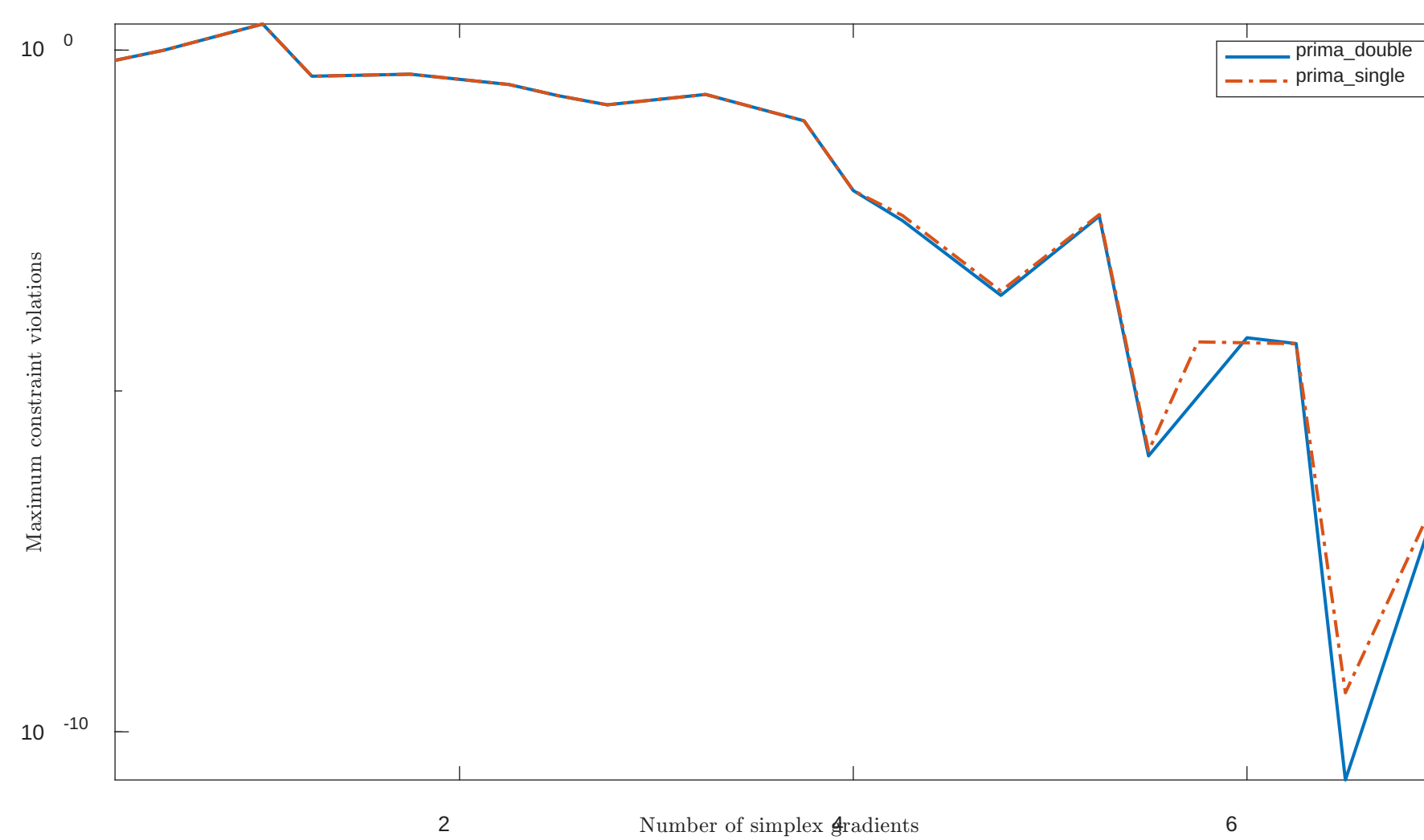
Solving "EIGMAXA" with "plain" feature
