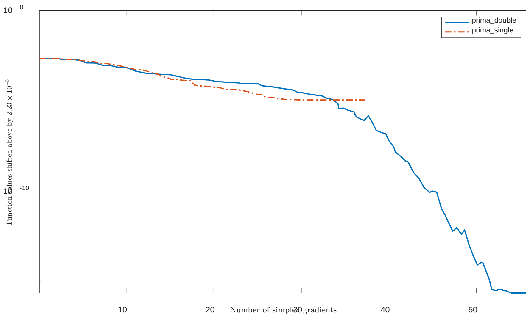
History profiles
