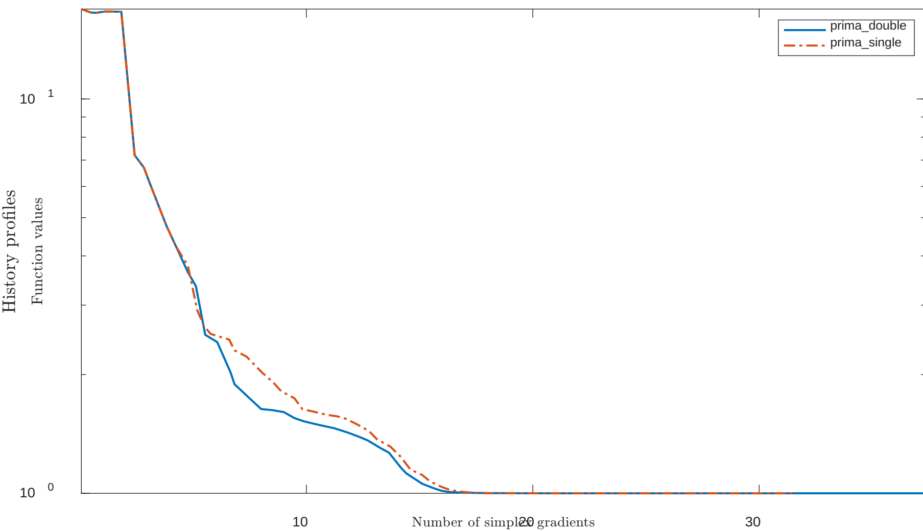
Solving “FMINSRF2” with “plain” feature
