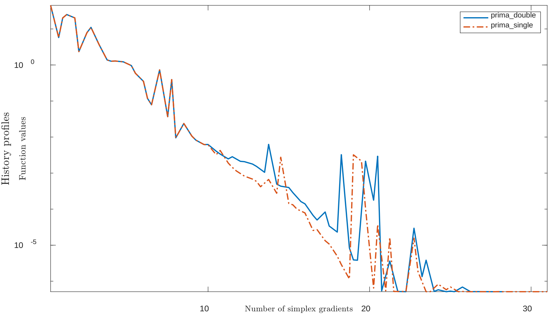
Solving “HATFLDE” with “plain” feature
