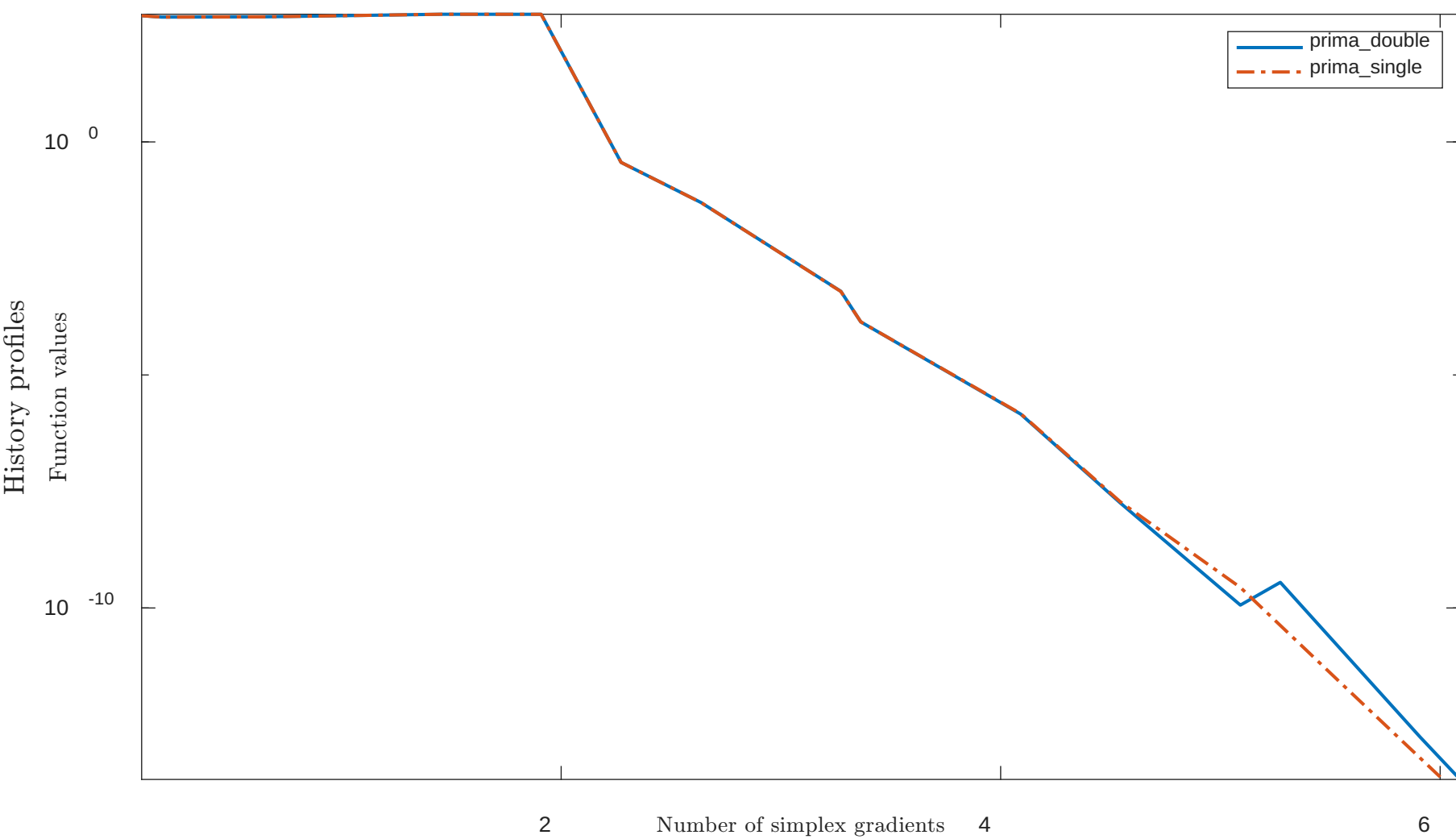
Solving “HILBERTB” with “plain” feature
